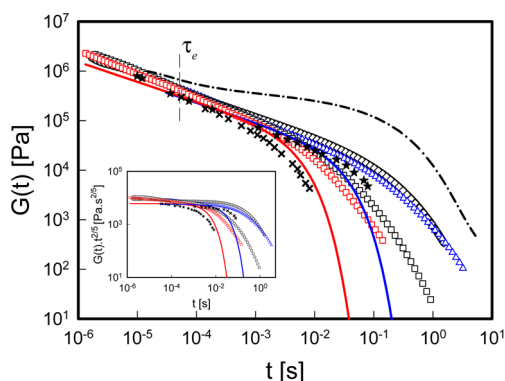
Figure 2. Stress relaxation modulus for PI rings and PS rings at T - T_g = 65 °C. PI 81k (blue triangle); PI 38k (red square); PS198k (black diamond); PS160k (black square). The stars and the crosses are from molecular dynamic simulations on coarse-grained bead–spring rings with Z \approx 3.6 and 14.4 from ref 24 (see Supporting Information for details about the conversion of MD units into Pascals and seconds). The blue and the red lines are model predictions for PI 81k and 38k, respectively. The dash-dotted line is the relaxation modulus for the PI 81k linear polymer, exhibiting an entanglement plateau. The Rouse time for entanglements, \tau_e , of the linear PI81k is also depicted for reference. Inset: Scaled version of the same plot, without the linear polymer data for clarity (see text for details).
