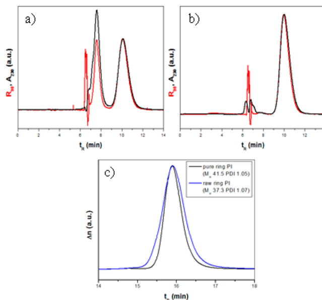
Figure 1. LCCC chromatograms for ring PI 38 kg/mol before (a) and after (b) LCCC fractionation. (c) SEC chromatograms before (blue) and after (black) LCCC fractionation.
