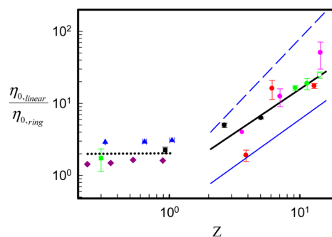
Figure 3. Ratio of the zero shear viscosities of linear and ring polymers as a function of the number of entanglements. The black dotted horizontal line sets the theoretical value of 2 in the low- Z region. The black continuous line is the best fit of the experimental data (slope of 1.2 \pm 0.3 ). The continuous and dashed blue lines have slopes of 1.3 and 1.9, respectively (see text for details). black circle, PEO experimental data set (Table 1); red circle, PI experimental data set (Table 1); green open circle, PS experimental data point (Table 1); 22,23 green filled circle, PS experimental data set from ref 3; black square, PEO experimental data point; 27 green square, PS experimental data point (Table 1); 28 purple diamond, PEO experimental data set; 29 blue triangle, polyethylene (PE) atomistic simulations; 30 pink circle, MD simulations on coarse-grained bead–spring chains. 24
